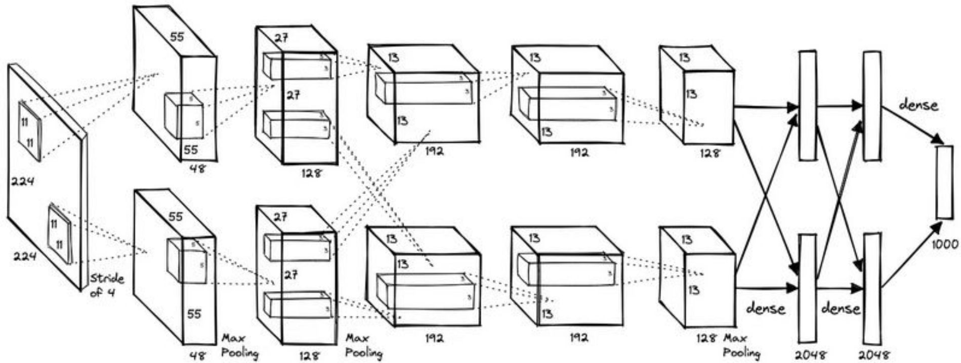
Network architecture of AlexNet [1].
